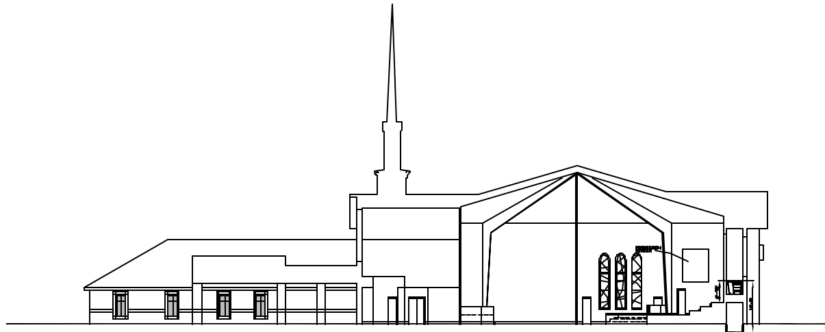
A BUILDING SECTION SCALE: 3/8" = 1'-0"
